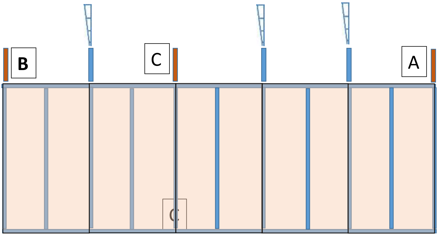
Rear Elevation – all full width sheets 8'x4'
